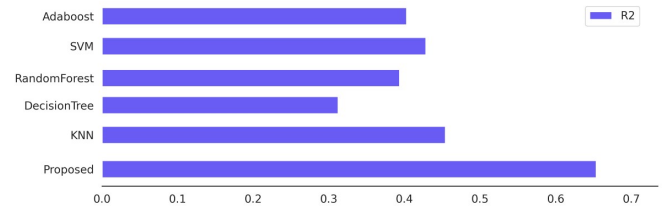
Fig. 10 Results of the R^2 for various models
